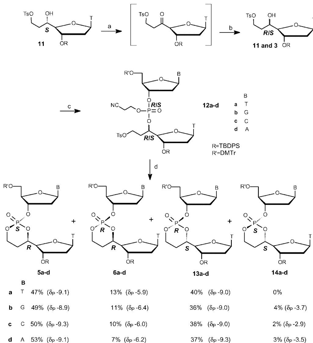
Scheme 2. Diastereoselective synthesis of the ( R C5' , S P )-, ( R C5' , R P )-, ( S C5' , R P )- and ( S C5' , S P )-configured \alpha,\beta -D-CNA XT dimers (X = T, G, C and A). Reagents and conditions: (a) PDC (pyridinium dichromate), CH 2 Cl 2 , room temp. (b) NaBH 4 , EtOH, 0 °C, 90%. (c) 5'- O -Dimethoxytrityl-3'- O -phosphoramidite-nucleoside (T, G, C and A), tetrazole, CH 3 CN, then collidine, I 2 /H 2 O, 67–92%. (d) K 2 CO 3 , DMF, room temp., 84–95%.
