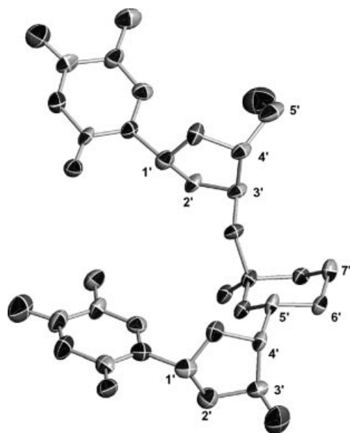
Figure 4. X-ray molecular structure of the ( R_{C5',Sp} )-configured \alpha,\beta -D-CNA TT dimer 9 with the adopted numbering scheme, displaying the chair and C2'-endo conformations of the dioxaphosphorinane and sugar subunits. For clarity, hydrogen atoms and cocrystallized solvent molecules are omitted, and thermal ellipsoids are shown at 40% probability.
