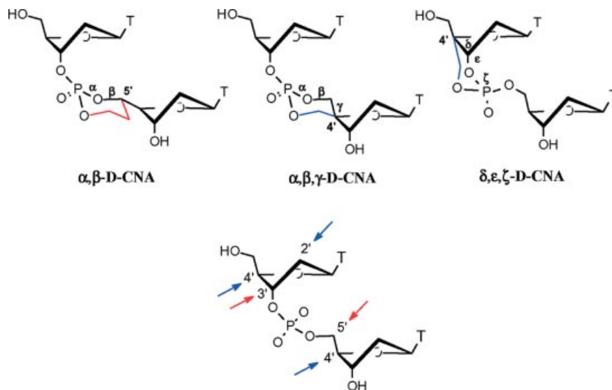
Figure 2. Example of previously described D-CNA dimeric units. D-CNA are oligonucleotides that contain one or more D-CNA dimers, in which a set of backbone torsion angles \alpha – \zeta is stereocontrolled to canonical or noncanonical values by a 1,3,2-dioxaphosphorinane ring structure. For a given dinucleotide step, there are fourteen possible [ \beta -D-deoxyribo]-configured D-CNA stereoisomers, which formally result from the introduction of a methylene/ethylene linker between the nonbridging phosphate oxygen atoms and the 2'/4'-carbon atoms (methylene linker, blue arrows) or 3'/5'-carbon atoms (ethylene linker, red arrows).
