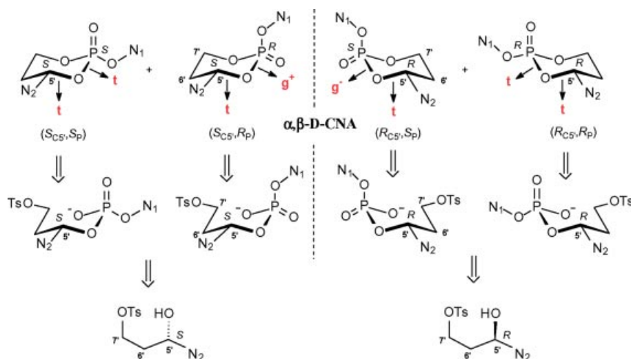
Figure 3. Retrosynthetic pathway for the diastereoselective synthesis of the four possible stereoisomers of \alpha,\beta -D-CNA dimers. N 1 and N 2 stand for the remaining atomic fragments that define the upper and lower nucleoside units, respectively. The expected gauche(+), gauche(–), or trans conformations of \alpha (P–O5') and \beta (O–C5') are indicated for the hypothetical true chair conformations associated with each diastereoisomer.
