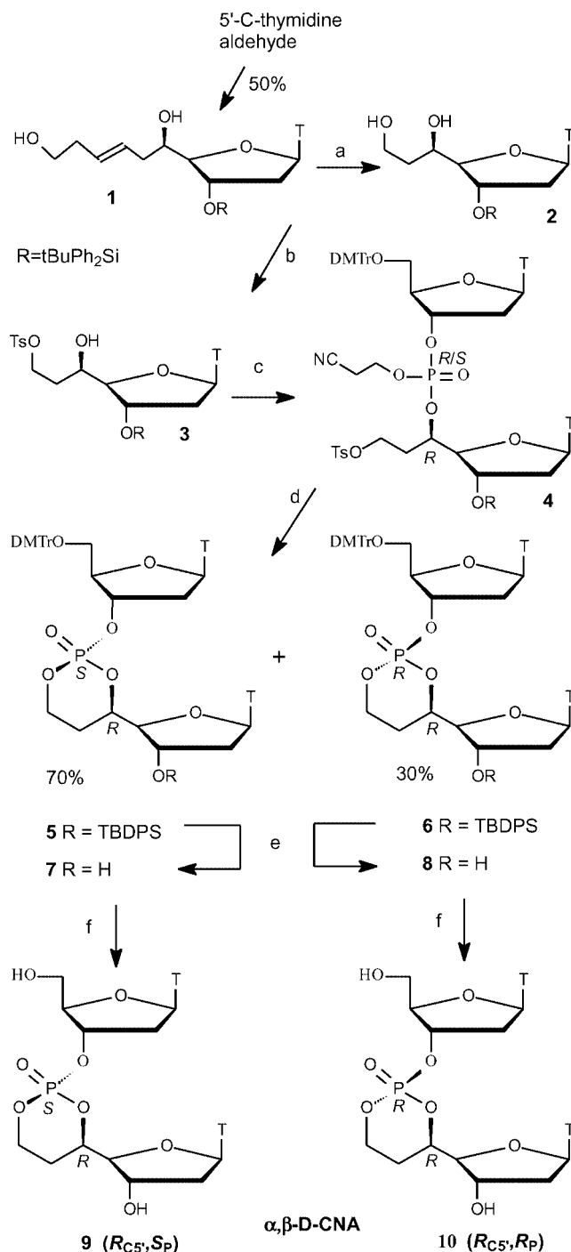
Scheme 1. Diastereoselective synthesis of the ( R C5' , S P )- and ( R C5' , R P )-configured \alpha,\beta -D-CNA TT dimers. Reagents and conditions: (a) i) OsO 4 cat., N -methylmorpholine N -oxide, H 2 O. ii) NaIO 4 , MeOH. iii) NaBH 4 , EtOH, 64% overall yield. (b) TsCl, Pyr, CHCl 3 , 77%. (c) 5'- O -Dimethoxytrityl-3'- O -phosphoramidite-thymidine, tetrazole, CH 3 CN, then collidine, I 2 /H 2 O, 93%. (d) Et 3 N, DMF, 90 °C, 90%. (e) n Bu 4 NF, THF, 86–90%. (f) 3% TFA in CH 2 Cl 2 , 77–85%.
